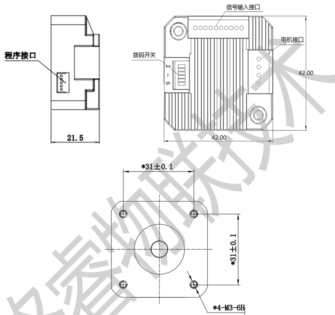
Figure 2.1 Installation dimensions (unit: mm)
